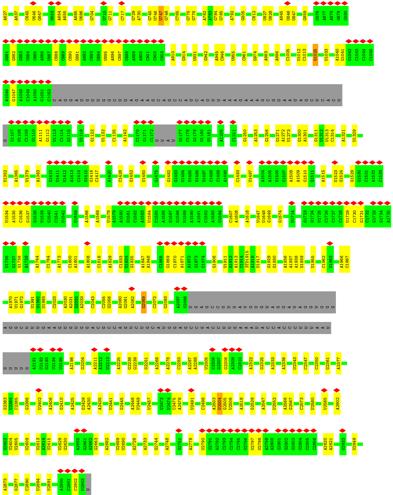
• Molecule 23: 5S rRNA
