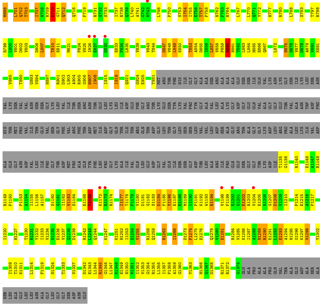
• Molecule 3: DNA-directed RNA polymerase subunit beta'
